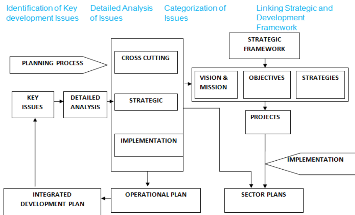
Figure 38: Planning Process
